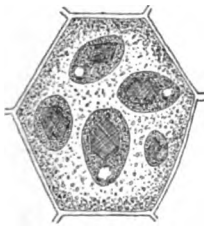
FIG. 66. — A cell from Castor Bean, showing the protein grains, of which the structure is rendered visible by treatment with reagents.
